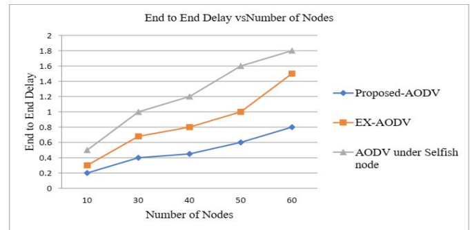
Figure 6: End-to-end Delay vs Number of Nodes.
