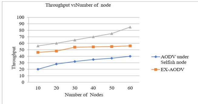
Figure 8: Throughput vs Number of nodes.
