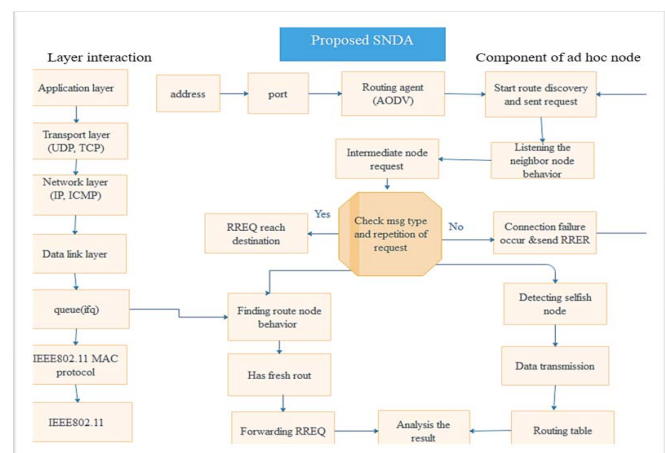
Figure 3: Flow Chart of Proposed SFNDA Algorithm.
