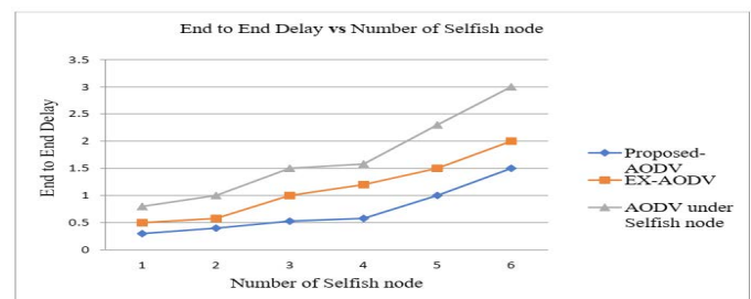
Figure 7: End-to-end Delay vs Number of Selfish nodes.
