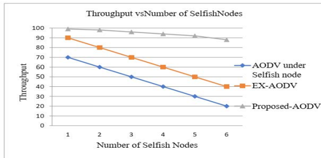
Figure 9: Throughput vs Number of Selfish Nodes.
