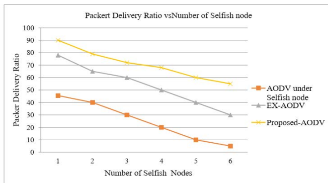
Figure 5: Packet Delivery Ratio vs Number of Selfish Nodes.
