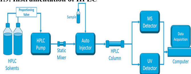
Figure1: Schematic diagram of HPLC instrumentation
