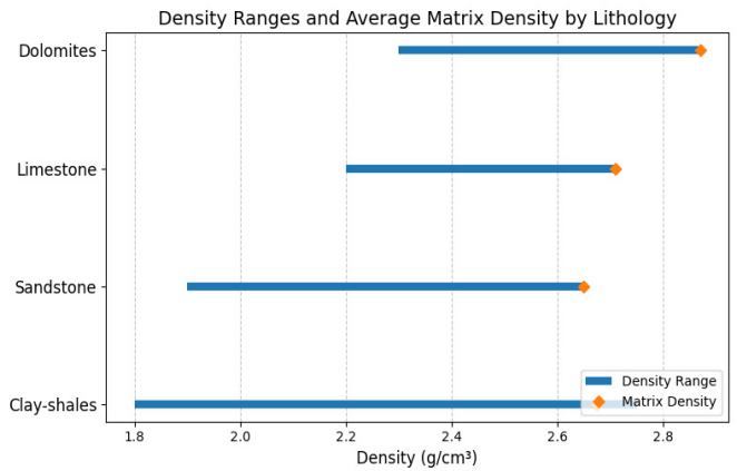
Figure 2: Densities of common lithologies (After, 1989)
