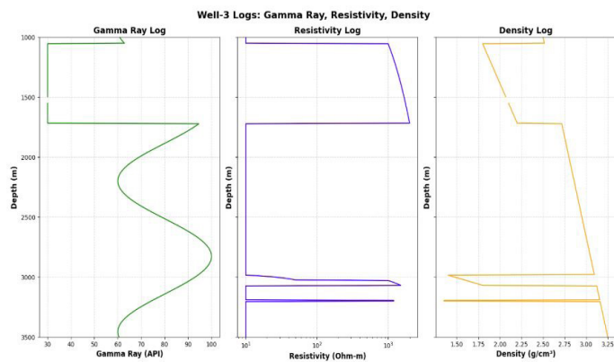
Figure 6: Gamma Ray Resistivity and Density logs of Well 3.
