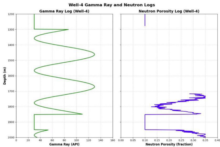
Figure 7: Gamma Ray and Neutron logs of Well 4.
