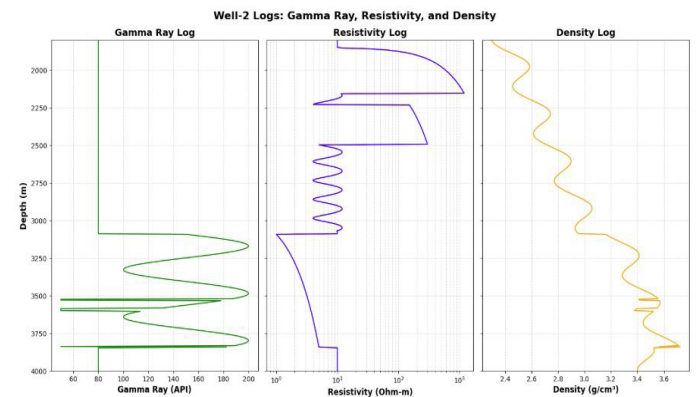
Figure 5: Gamma Ray, Resistivity and Density logs of Well 2
