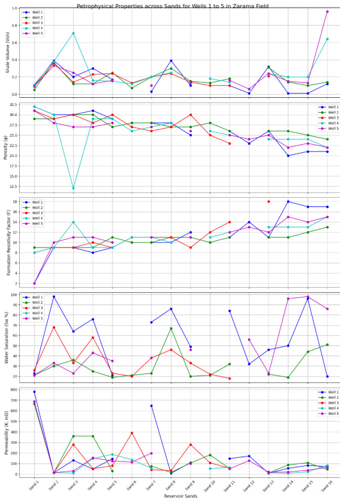
Figure 10: Comparison of Petrophysical Analysis in the study area.
