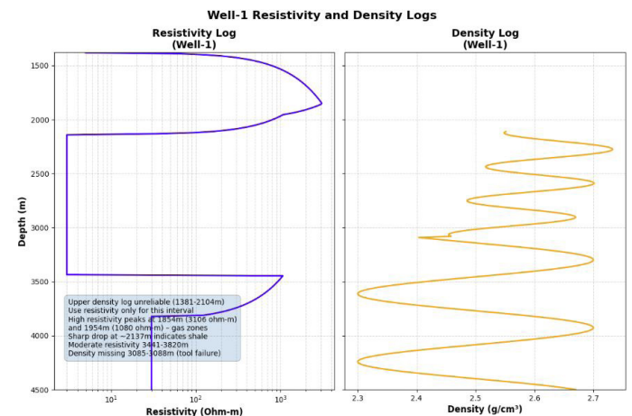
Figure 4: Resistivity and Density logs of Well 1.
