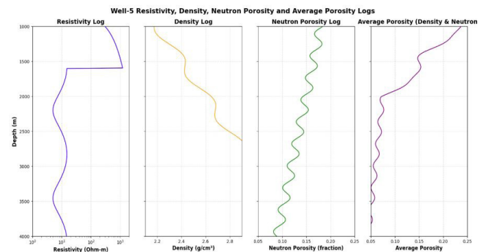
Figure 8: Resistivity, Neutron, Porosity and Average Logs.
