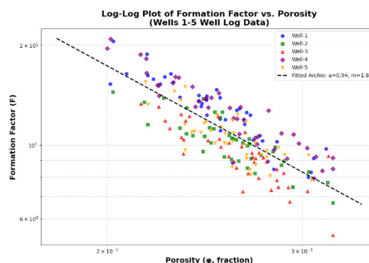
Figure 13: Log-log plot of Formation Factor as a function of Porosity for the Wells applying the equation \log(F) = \log(a) - m \log(\phi) derived from Archie's Formation factor equation F = a \phi^{-m} to the study area
