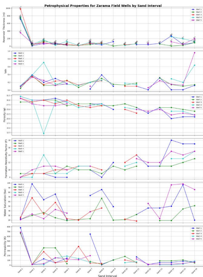
Figure 9: Results of Petrophysical Analysis of Sands S1 to S16 of the study Area.
